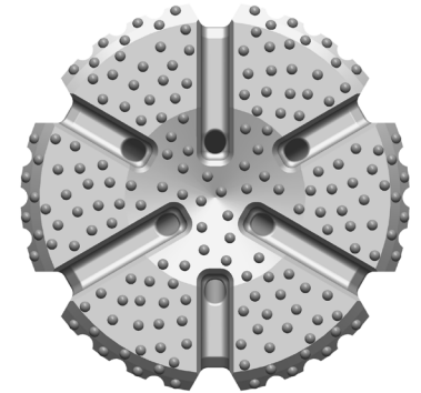
Concave/Plate
